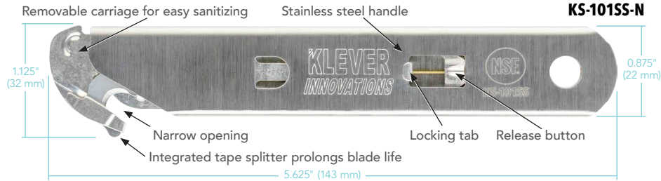
KS-101SS-N Narrow Opening (0.125" / 3 mm)
