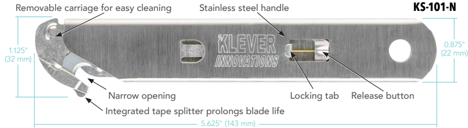
KS-101-N Narrow Opening (0.125" / 3 mm)
